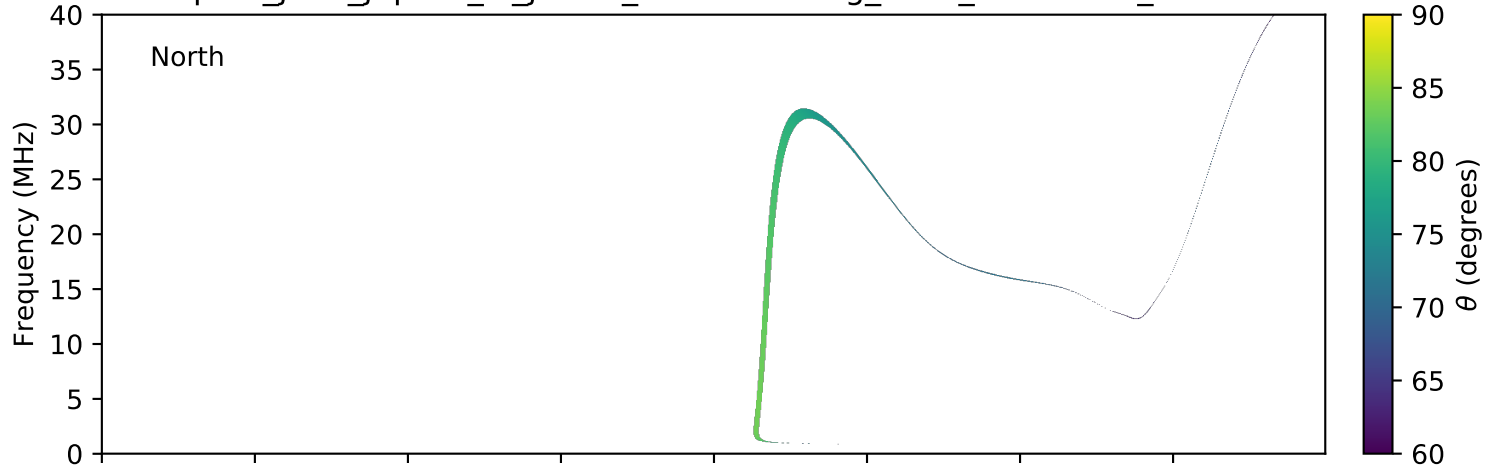
expres_juno_jupiter_io_jrm09_lossc-wid1deg_3kev_20180711_v01.cdf
