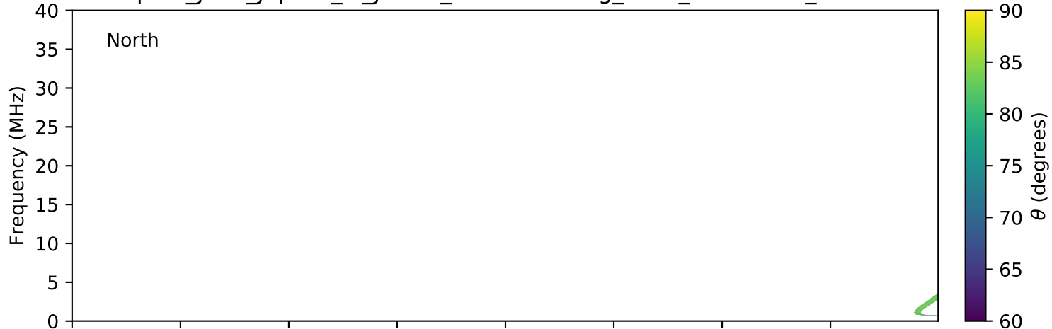
expres_juno_jupiter_io_jrm09_lossc-wid1deg_3kev_20180707_v01.cdf
