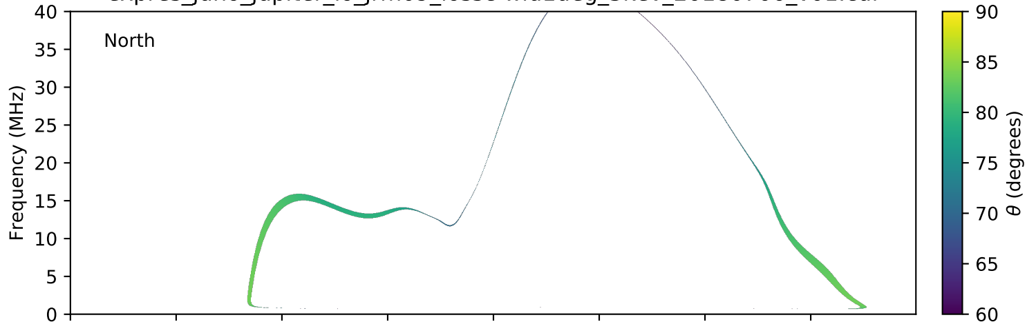
expres_juno_jupiter_io_jrm09_lossc-wid1deg_3kev_20180706_v01.cdf
