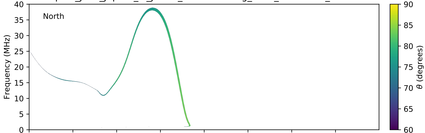
expres_juno_jupiter_io_jrm09_lossc-wid1deg_3kev_20180703_v01.cdf
