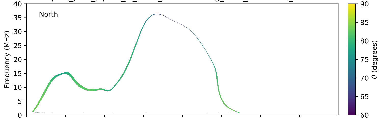
expres_juno_jupiter_io_isaac_lossc-wid1deg_3kev_20180731_v01.cdf
