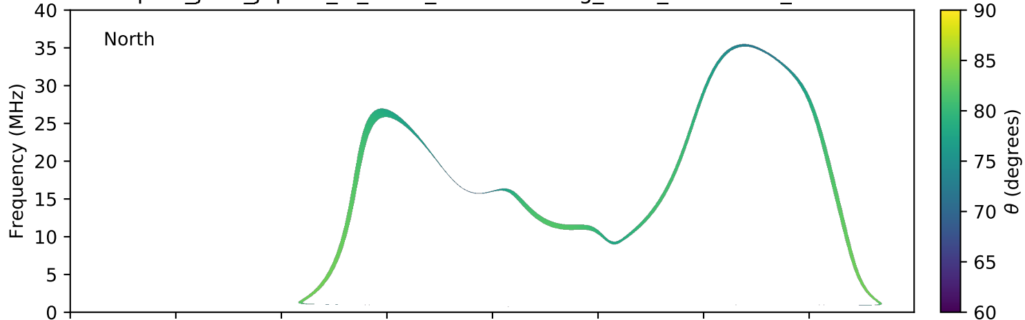
expres_juno_jupiter_io_isaac_lossc-wid1deg_3kev_20180729_v01.cdf
