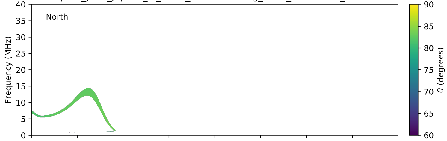
expres_juno_jupiter_io_isaac_lossc-wid1deg_3kev_20180728_v01.cdf
