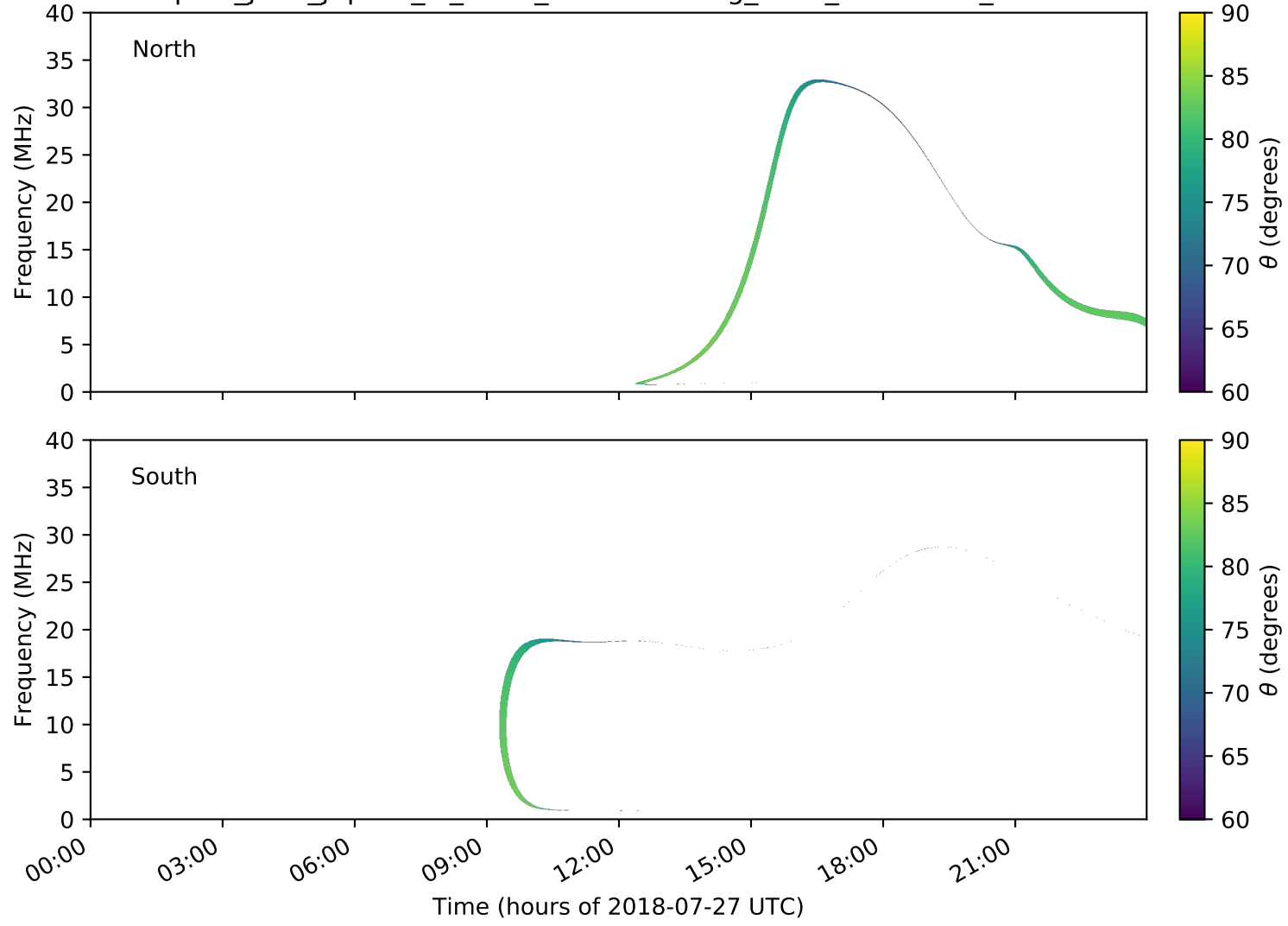
expres_juno_jupiter_io_isaac_lossc-wid1deg_3kev_20180727_v01.cdf
