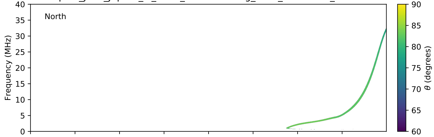
expres_juno_jupiter_io_isaac_lossc-wid1deg_3kev_20180725_v01.cdf
