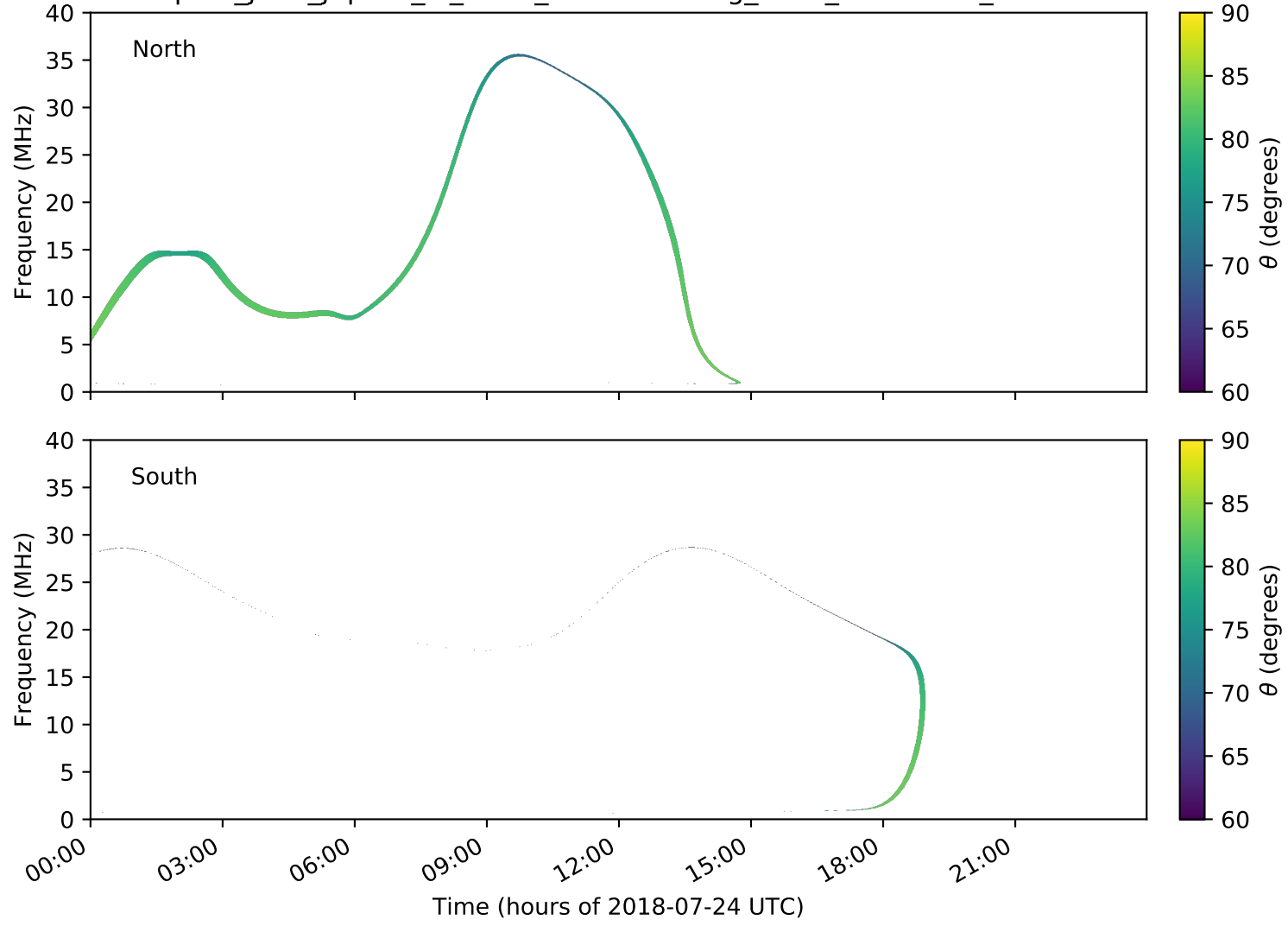
expres_juno_jupiter_io_isaac_lossc-wid1deg_3kev_20180724_v01.cdf
