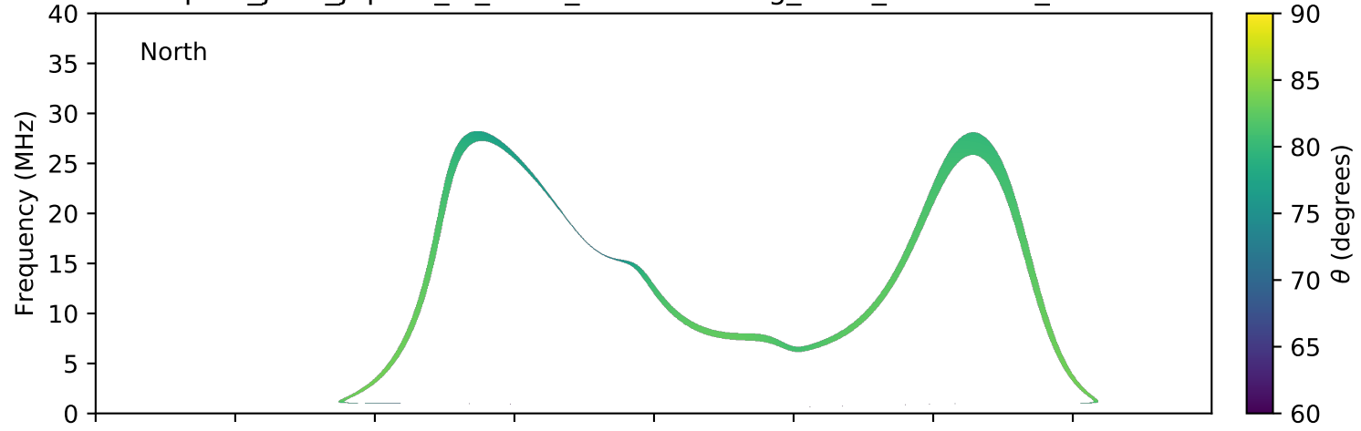
expres_juno_jupiter_io_isaac_lossc-wid1deg_3kev_20180722_v01.cdf
