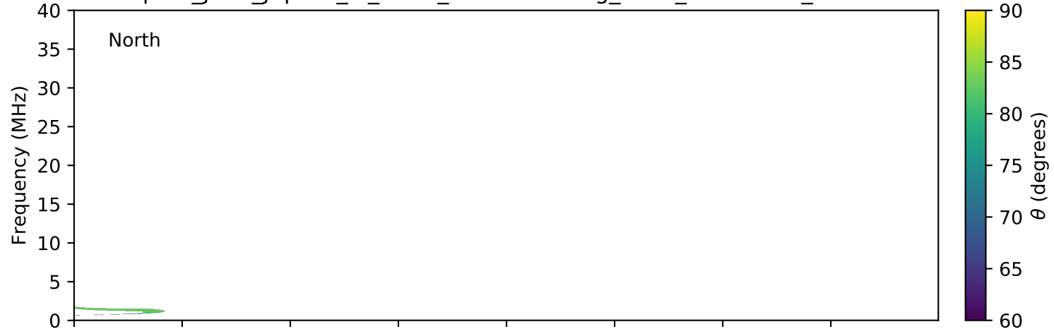
expres_juno_jupiter_io_isaac_lossc-wid1deg_3kev_20180721_v01.cdf
