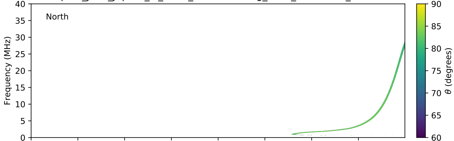
expres_juno_jupiter_io_isaac_lossc-wid1deg_3kev_20180718_v01.cdf
