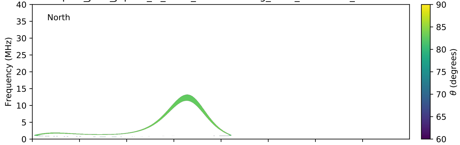
expres_juno_jupiter_io_isaac_lossc-wid1deg_3kev_20180717_v01.cdf
