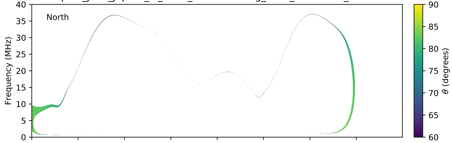
expres_juno_jupiter_io_isaac_lossc-wid1deg_3kev_20180715_v01.cdf
