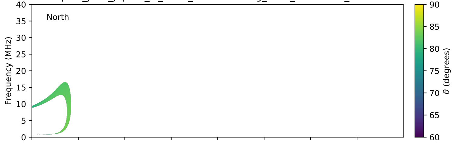
expres_juno_jupiter_io_isaac_lossc-wid1deg_3kev_20180714_v01.cdf
