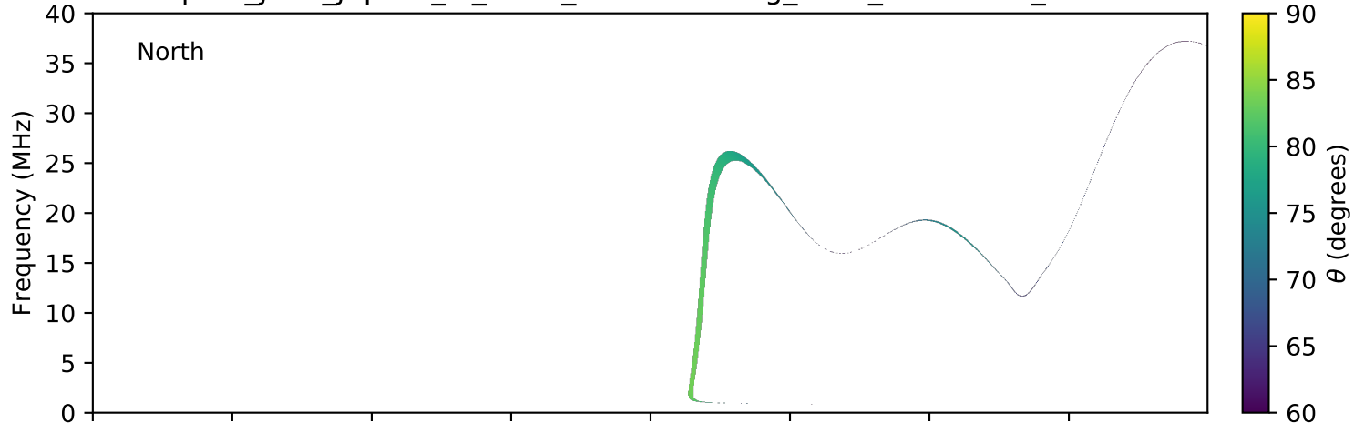
expres_juno_jupiter_io_isaac_lossc-wid1deg_3kev_20180711_v01.cdf
