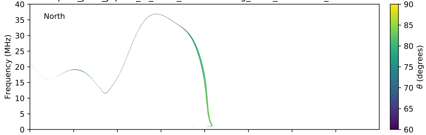
expres_juno_jupiter_io_isaac_lossc-wid1deg_3kev_20180710_v01.cdf
