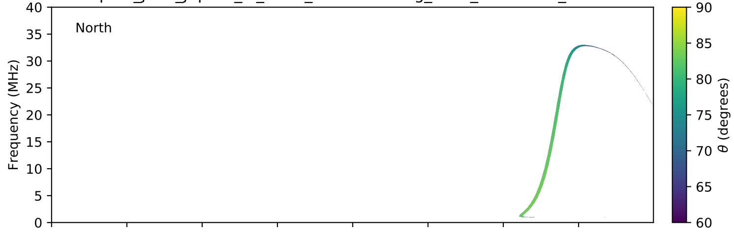
expres_juno_jupiter_io_isaac_lossc-wid1deg_3kev_20180709_v01.cdf
