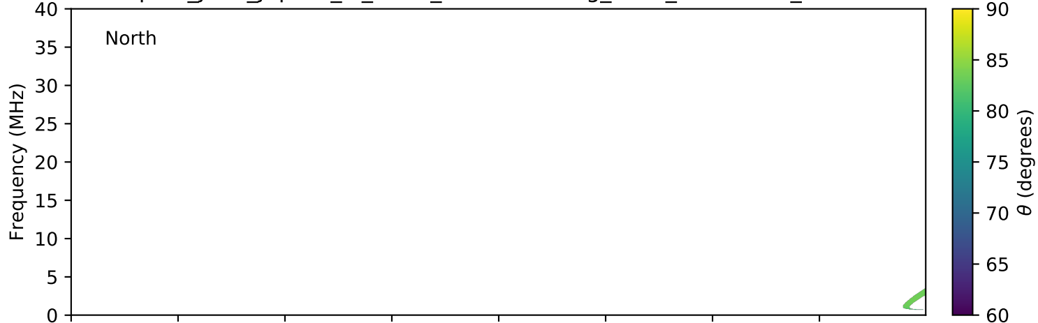
expres_juno_jupiter_io_isaac_lossc-wid1deg_3kev_20180707_v01.cdf
