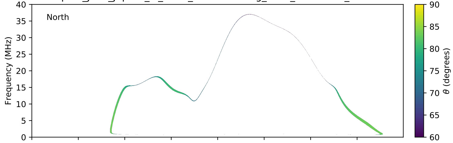
expres_juno_jupiter_io_isaac_lossc-wid1deg_3kev_20180706_v01.cdf
