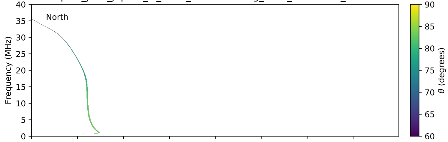
expres_juno_jupiter_io_isaac_lossc-wid1deg_3kev_20180705_v01.cdf
