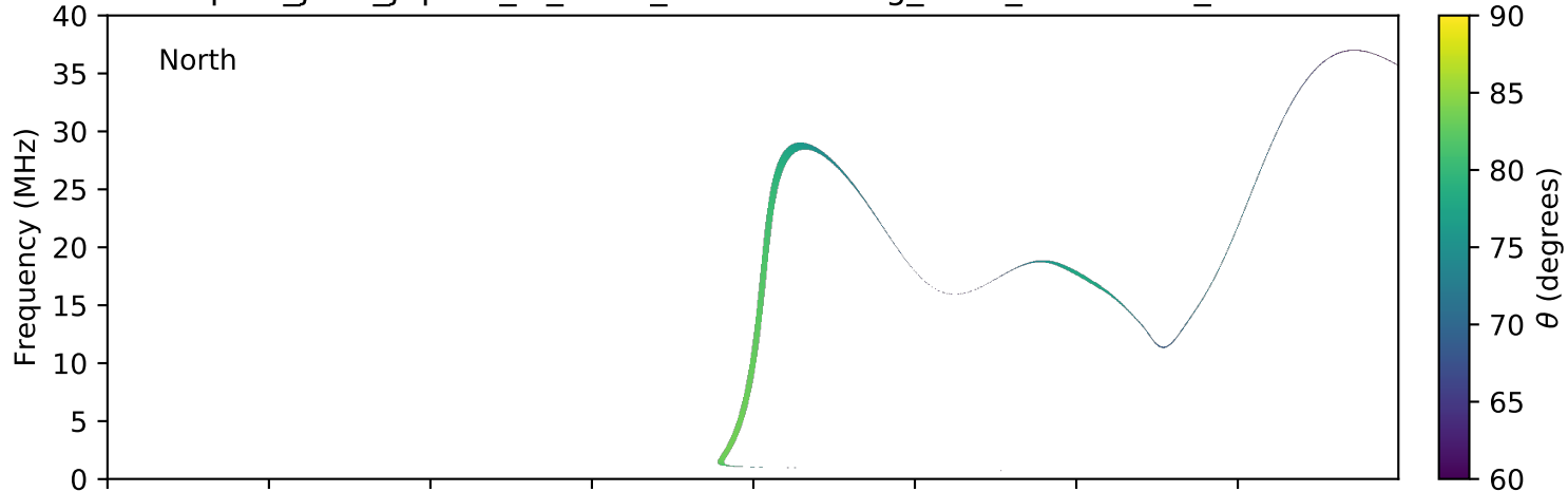
expres_juno_jupiter_io_isaac_lossc-wid1deg_3kev_20180704_v01.cdf
