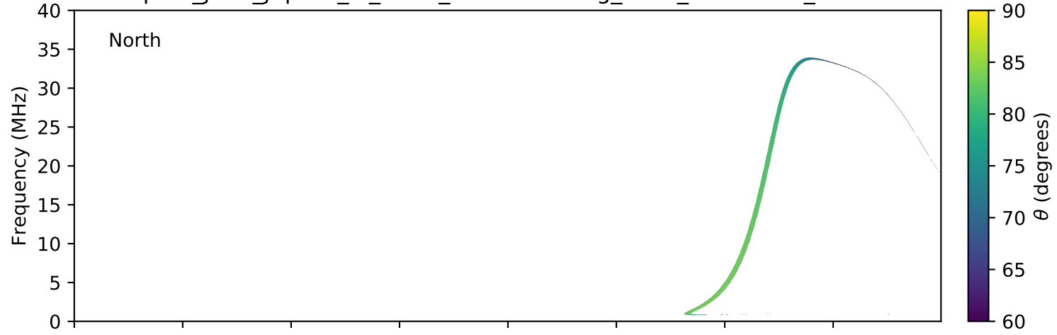
expres_juno_jupiter_io_isaac_lossc-wid1deg_3kev_20180702_v01.cdf
