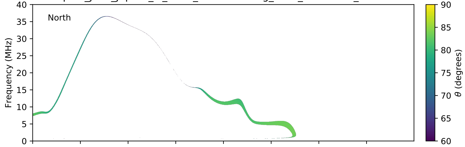
expres_juno_jupiter_io_isaac_lossc-wid1deg_3kev_20180701_v01.cdf
