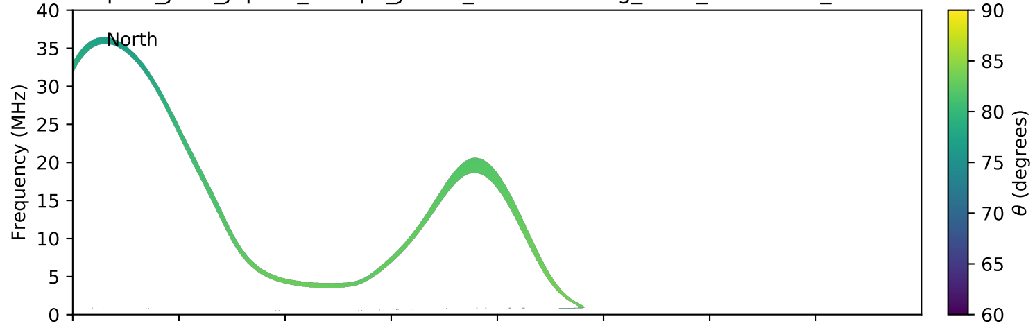
expres_juno_jupiter_europa_jrm09_lossc-wid1deg_3kev_20180731_v01.cdf
