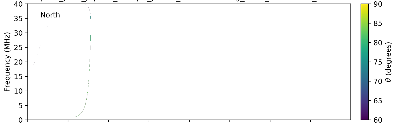
expres_juno_jupiter_europa_jrm09_lossc-wid1deg_3kev_20180716_v01.cdf
