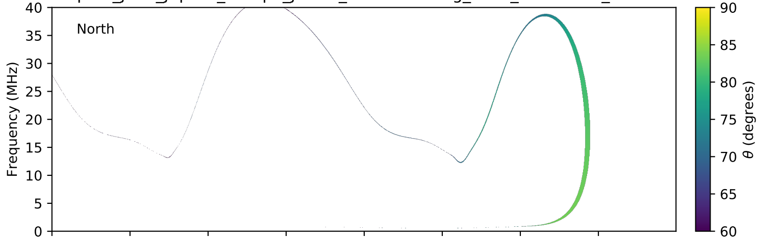
expres_juno_jupiter_europa_jrm09_lossc-wid1deg_3kev_20180715_v01.cdf
