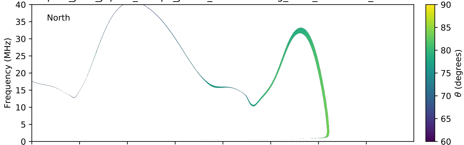
expres_juno_jupiter_europa_jrm09_lossc-wid1deg_3kev_20180713_v01.cdf
