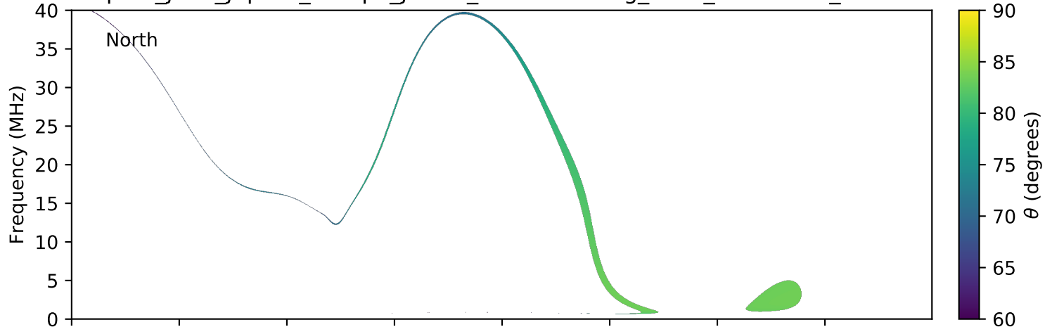
expres_juno_jupiter_europa_jrm09_lossc-wid1deg_3kev_20180712_v01.cdf
