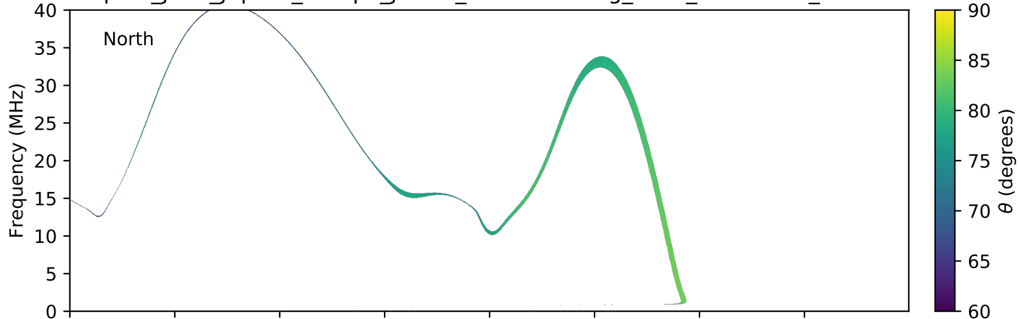
expres_juno_jupiter_europa_jrm09_lossc-wid1deg_3kev_20180711_v01.cdf
