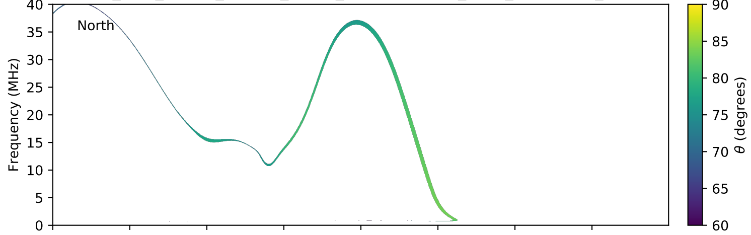
expres_juno_jupiter_europa_jrm09_lossc-wid1deg_3kev_20180707_v01.cdf
