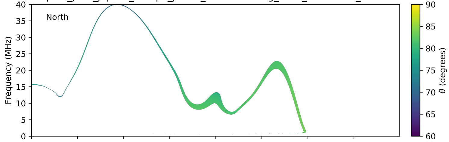
expres_juno_jupiter_europa_jrm09_lossc-wid1deg_3kev_20180706_v01.cdf
