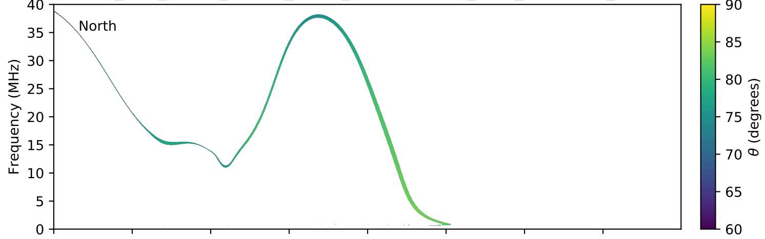
expres_juno_jupiter_europa_jrm09_lossc-wid1deg_3kev_20180705_v01.cdf
