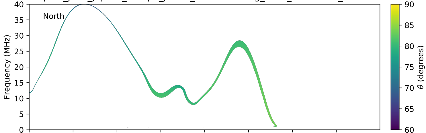
expres_juno_jupiter_europa_jrm09_lossc-wid1deg_3kev_20180704_v01.cdf
