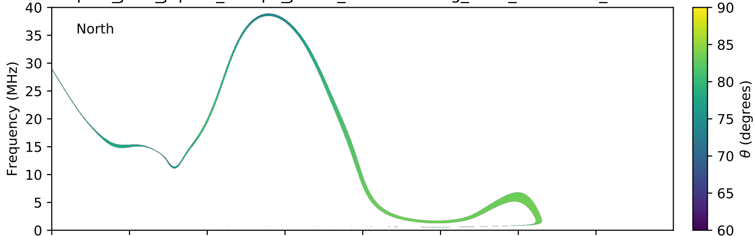
expres_juno_jupiter_europa_jrm09_lossc-wid1deg_3kev_20180703_v01.cdf
