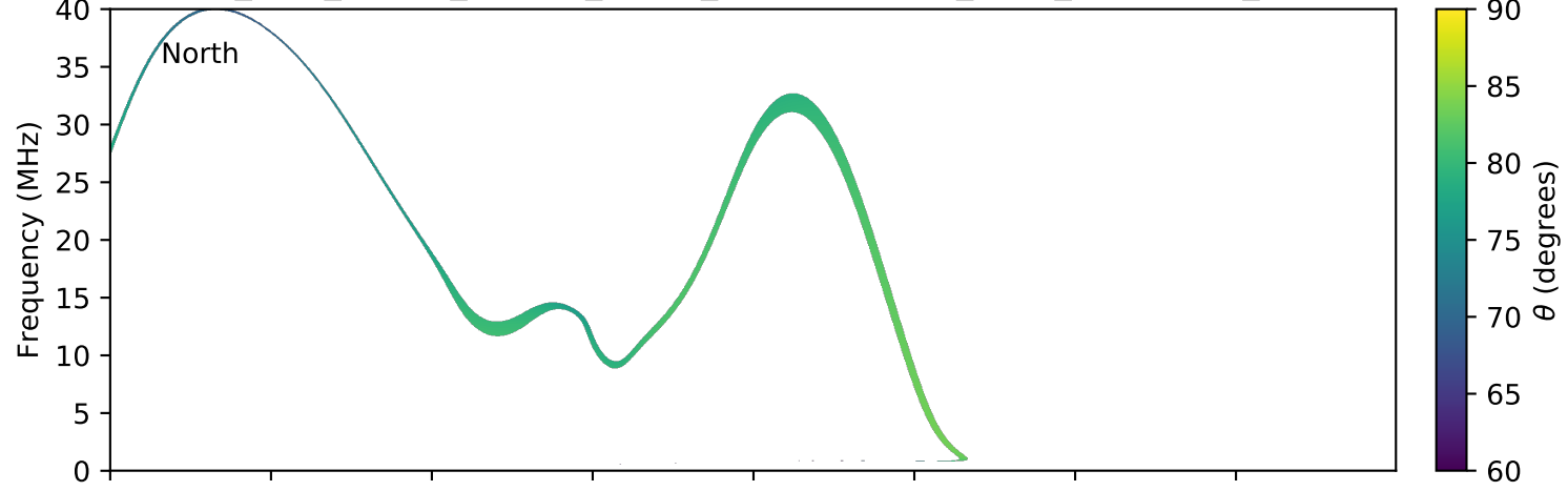
expres_juno_jupiter_europa_jrm09_lossc-wid1deg_3kev_20180702_v01.cdf
