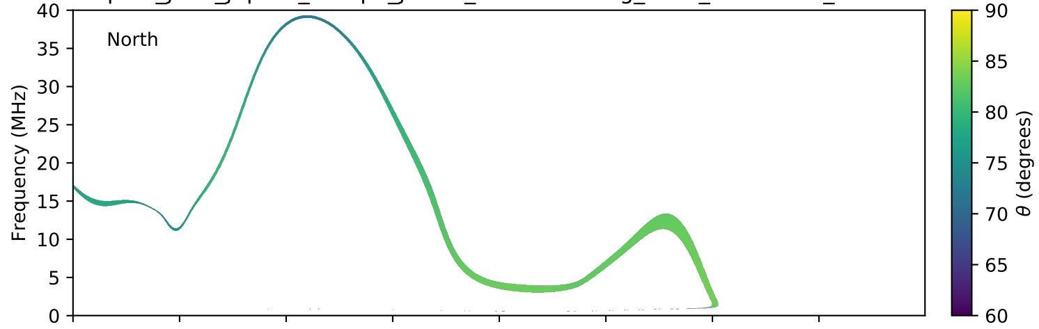
expres_juno_jupiter_europa_jrm09_lossc-wid1deg_3kev_20180701_v01.cdf
