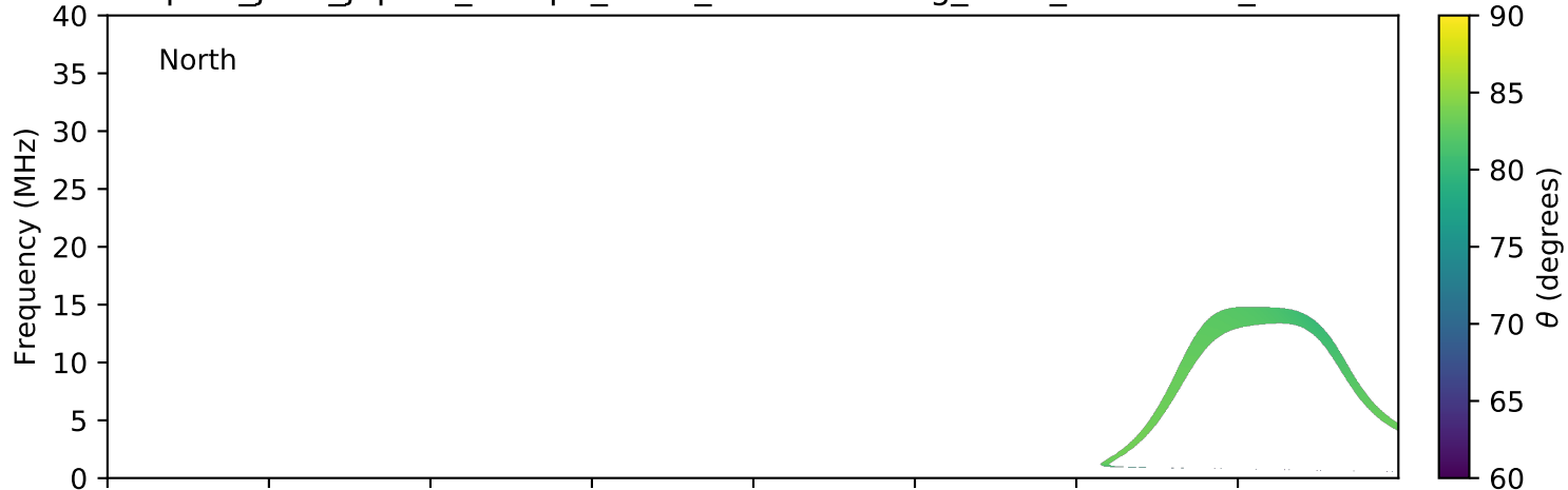
expres_juno_jupiter_europa_isaac_lossc-wid1deg_3kev_20180731_v01.cdf
