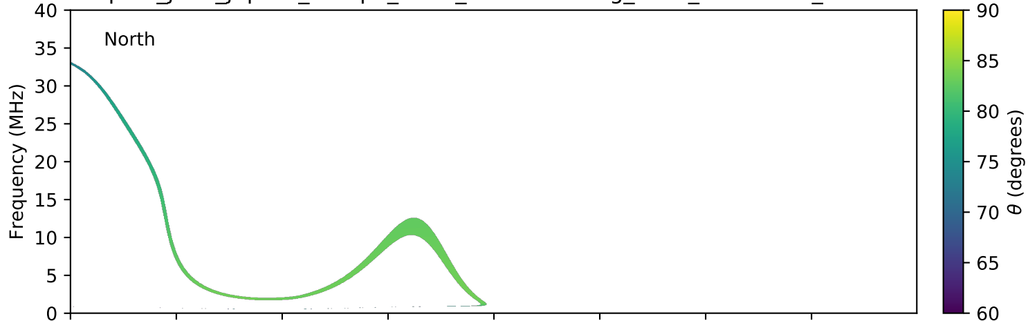
expres_juno_jupiter_europa_isaac_lossc-wid1deg_3kev_20180729_v01.cdf
