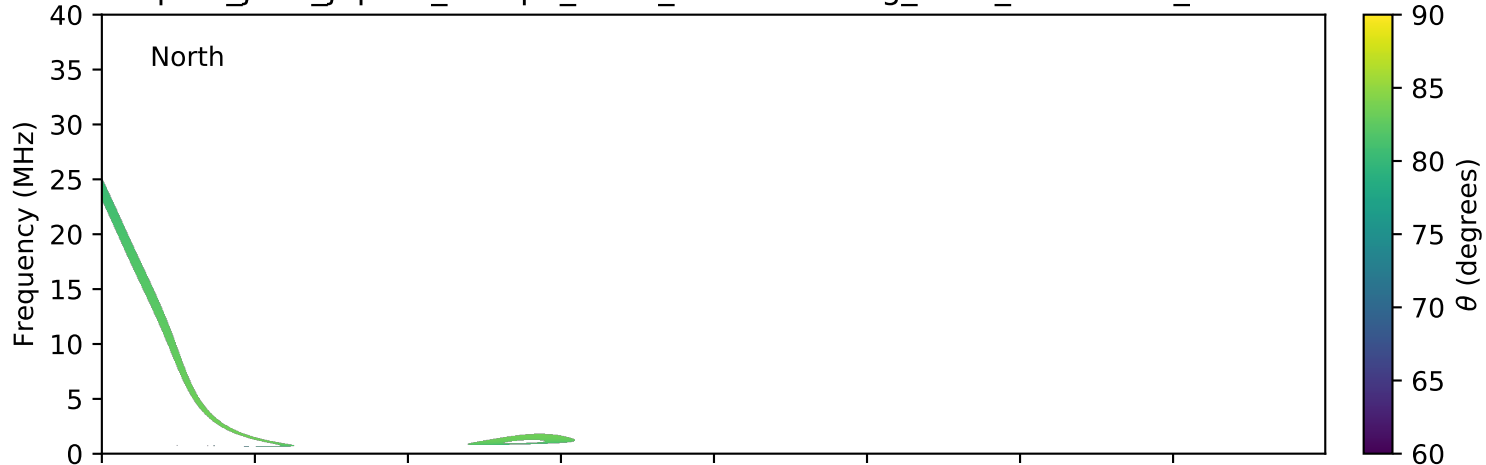
expres_juno_jupiter_europa_isaac_lossc-wid1deg_3kev_20180722_v01.cdf
