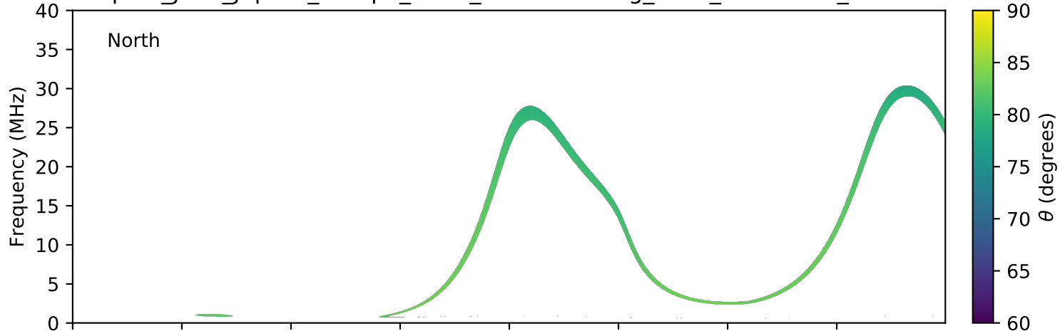
expres_juno_jupiter_europa_isaac_lossc-wid1deg_3kev_20180721_v01.cdf
