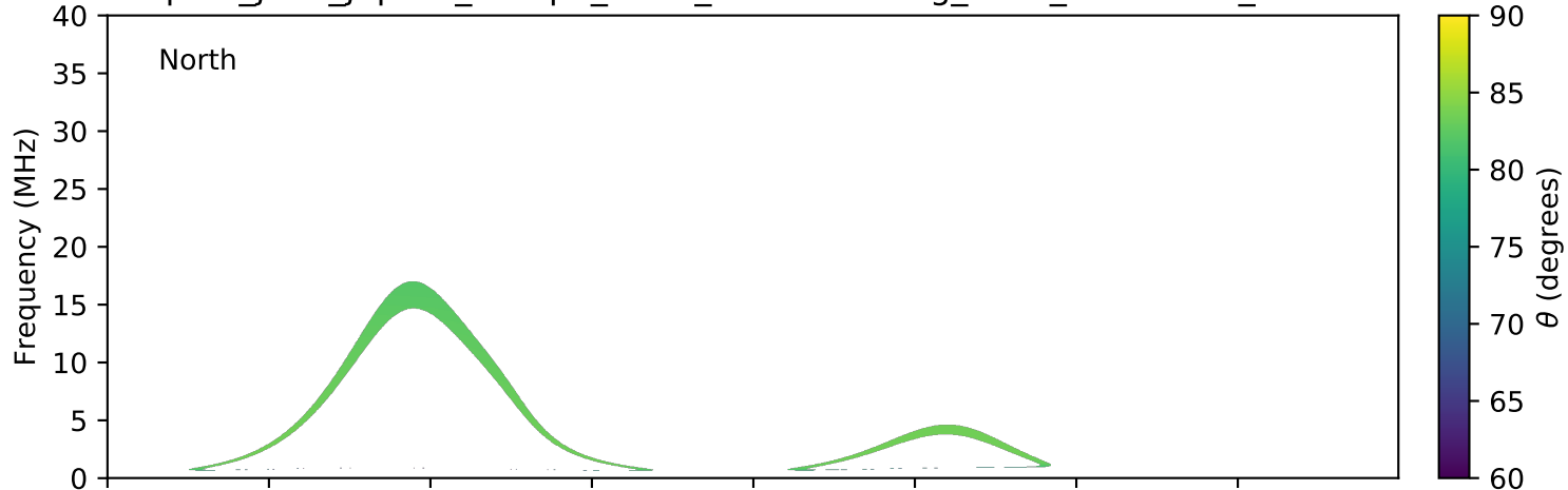
expres_juno_jupiter_europa_isaac_lossc-wid1deg_3kev_20180718_v01.cdf
