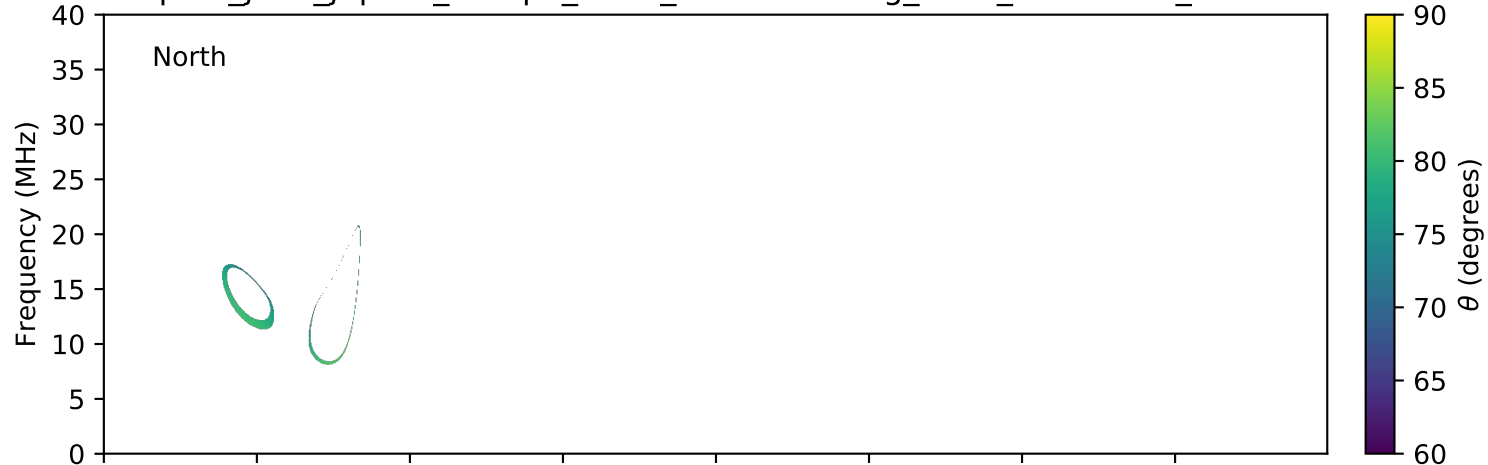
expres_juno_jupiter_europa_isaac_lossc-wid1deg_3kev_20180716_v01.cdf
