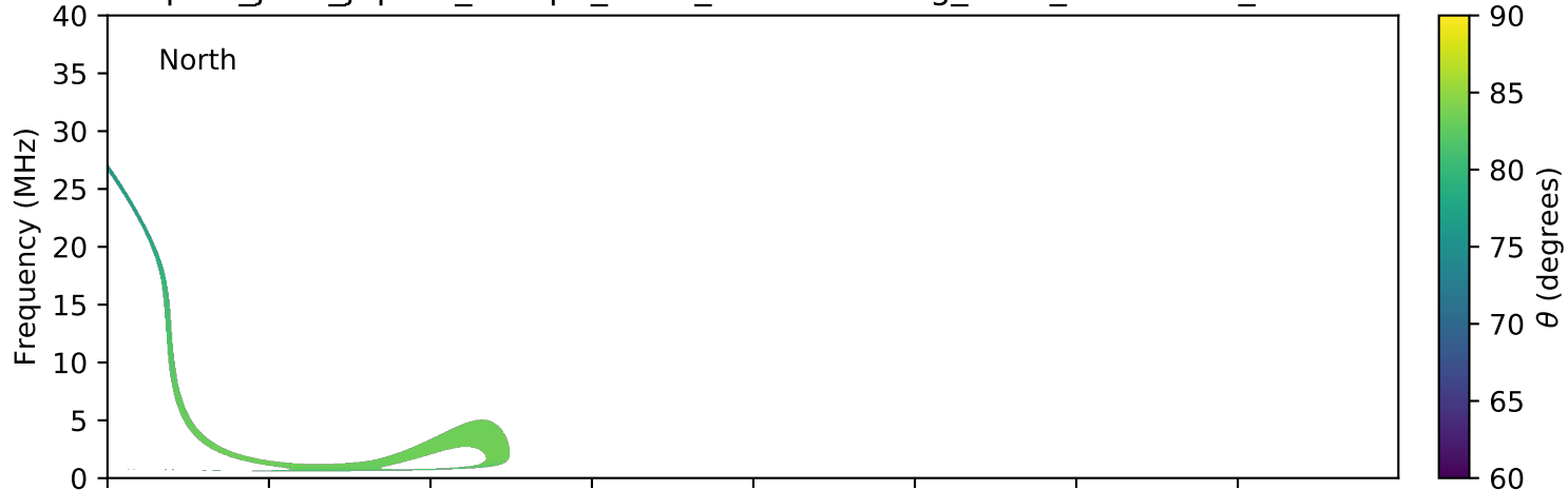
expres_juno_jupiter_europa_isaac_lossc-wid1deg_3kev_20180708_v01.cdf
