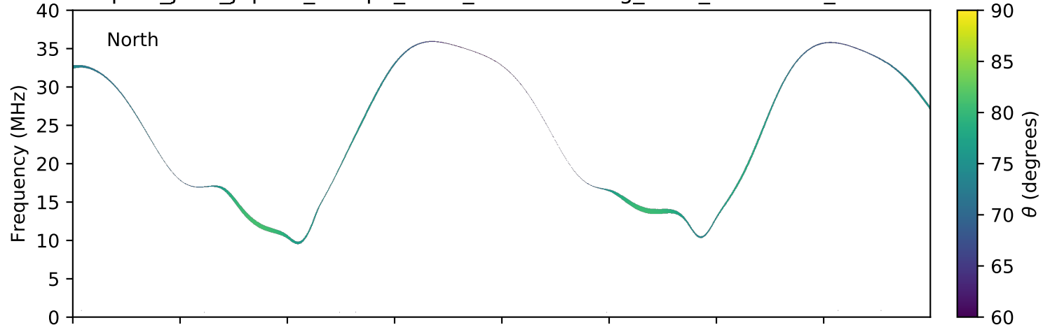
expres_juno_jupiter_europa_isaac_lossc-wid1deg_3kev_20180707_v01.cdf
