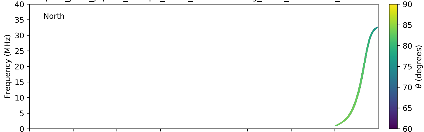
expres_juno_jupiter_europa_isaac_lossc-wid1deg_3kev_20180706_v01.cdf
