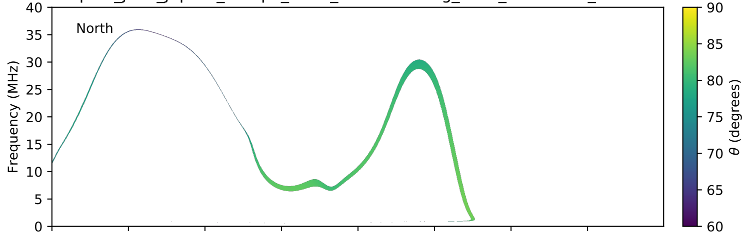
expres_juno_jupiter_europa_isaac_lossc-wid1deg_3kev_20180704_v01.cdf
