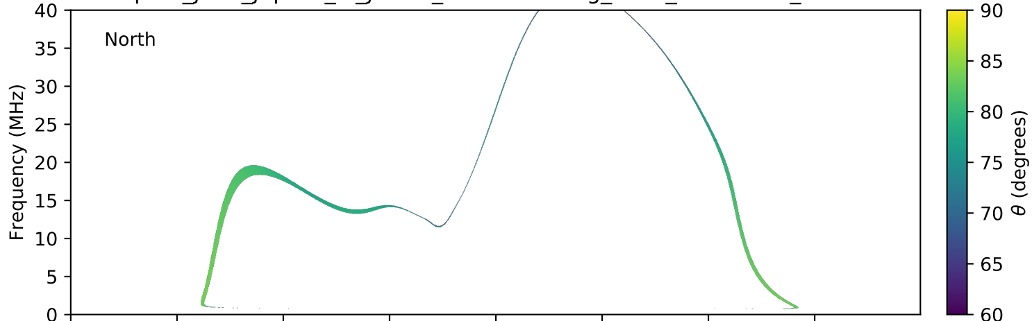
expres_juno_jupiter_io_jrm09_lossc-wid1deg_3kev_20180629_v01.cdf
