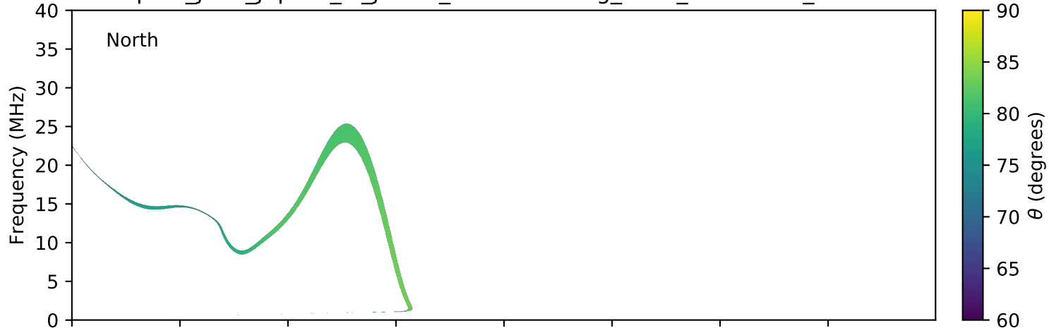
expres_juno_jupiter_io_jrm09_lossc-wid1deg_3kev_20180626_v01.cdf
